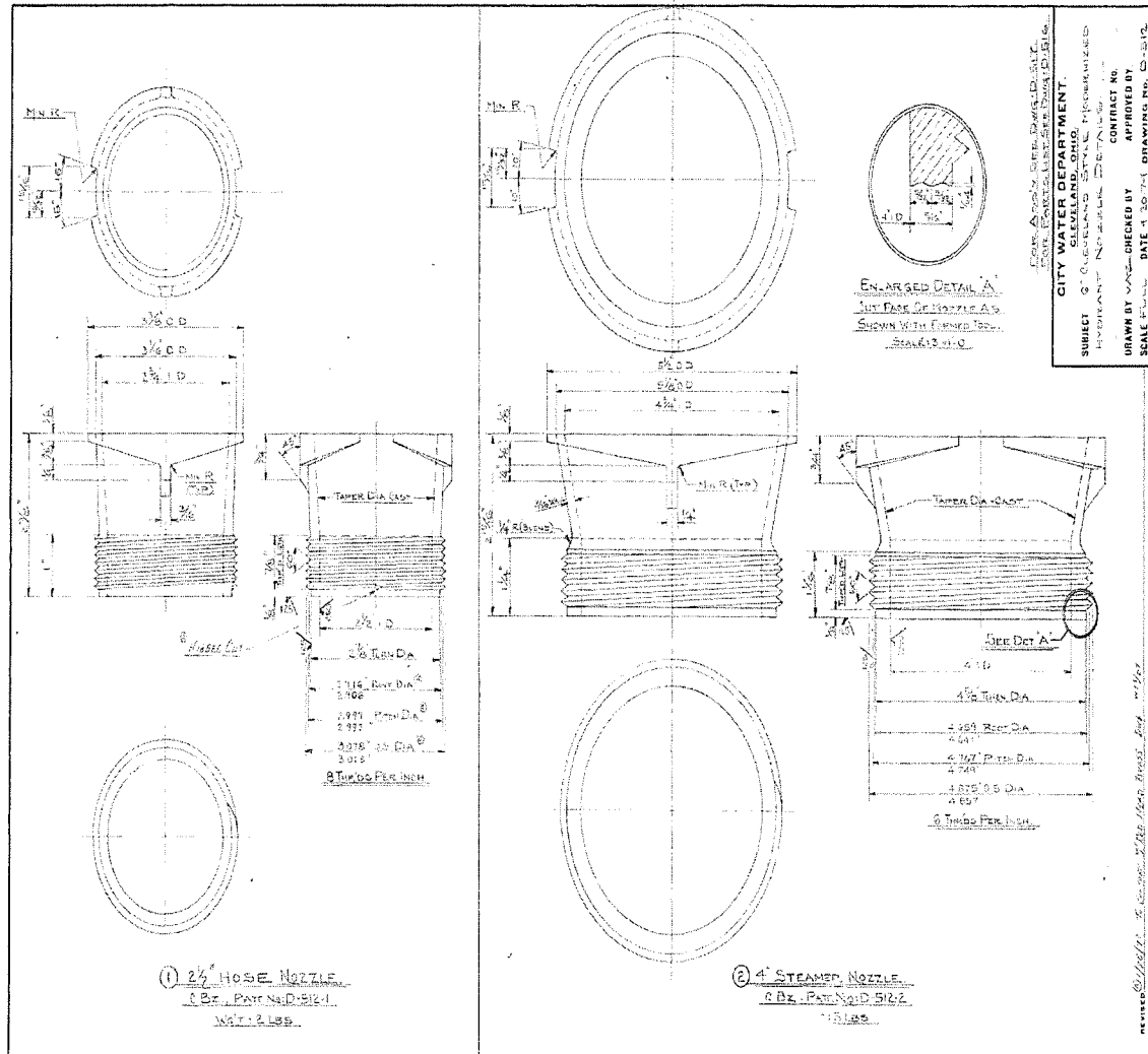
DRAWING D-512
