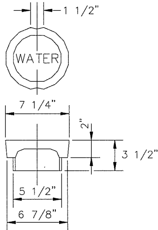
ALTERNATE COVER NO. 1
