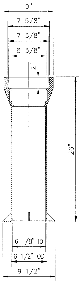
ALTERNATE LONG TOP NO. 2 WEIGHT 65 POUNDS
