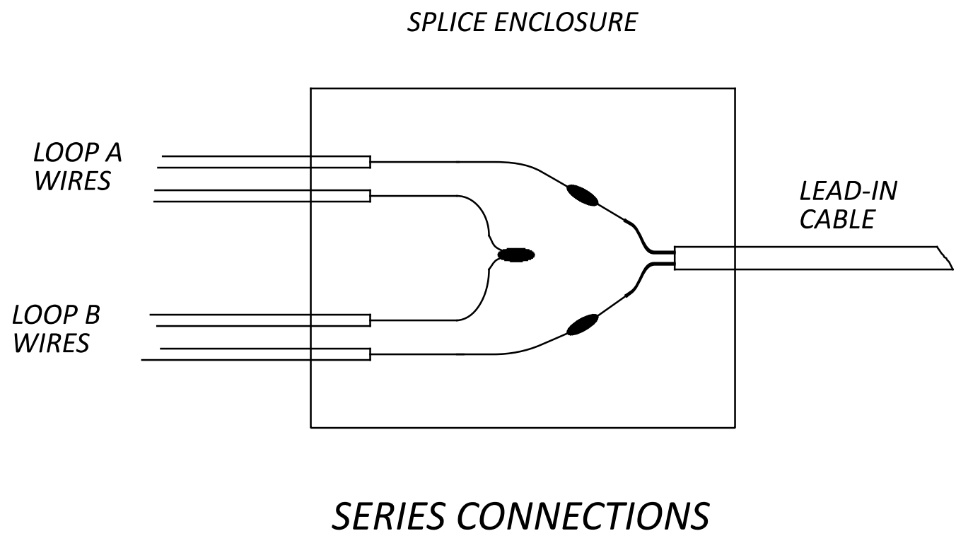
SERIES CONNECTIONS
