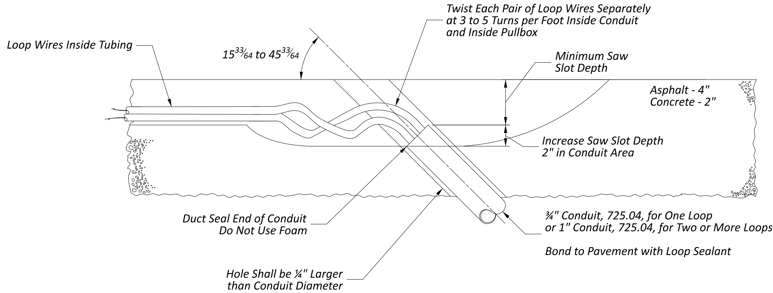
CONDUIT DRILLED HOLE DETAIL
