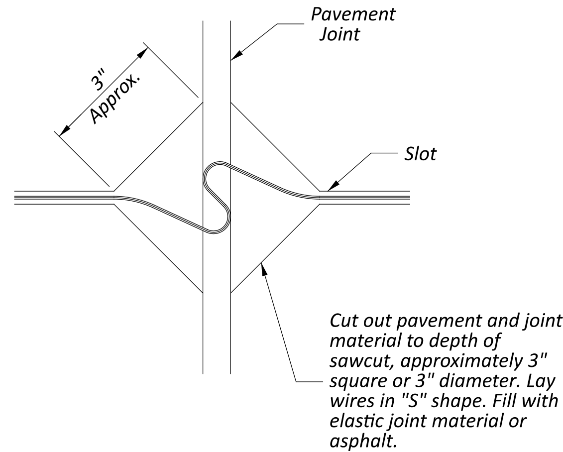
JOINT CROSSING DETAIL IN P.C.C. PAVEMENTS
