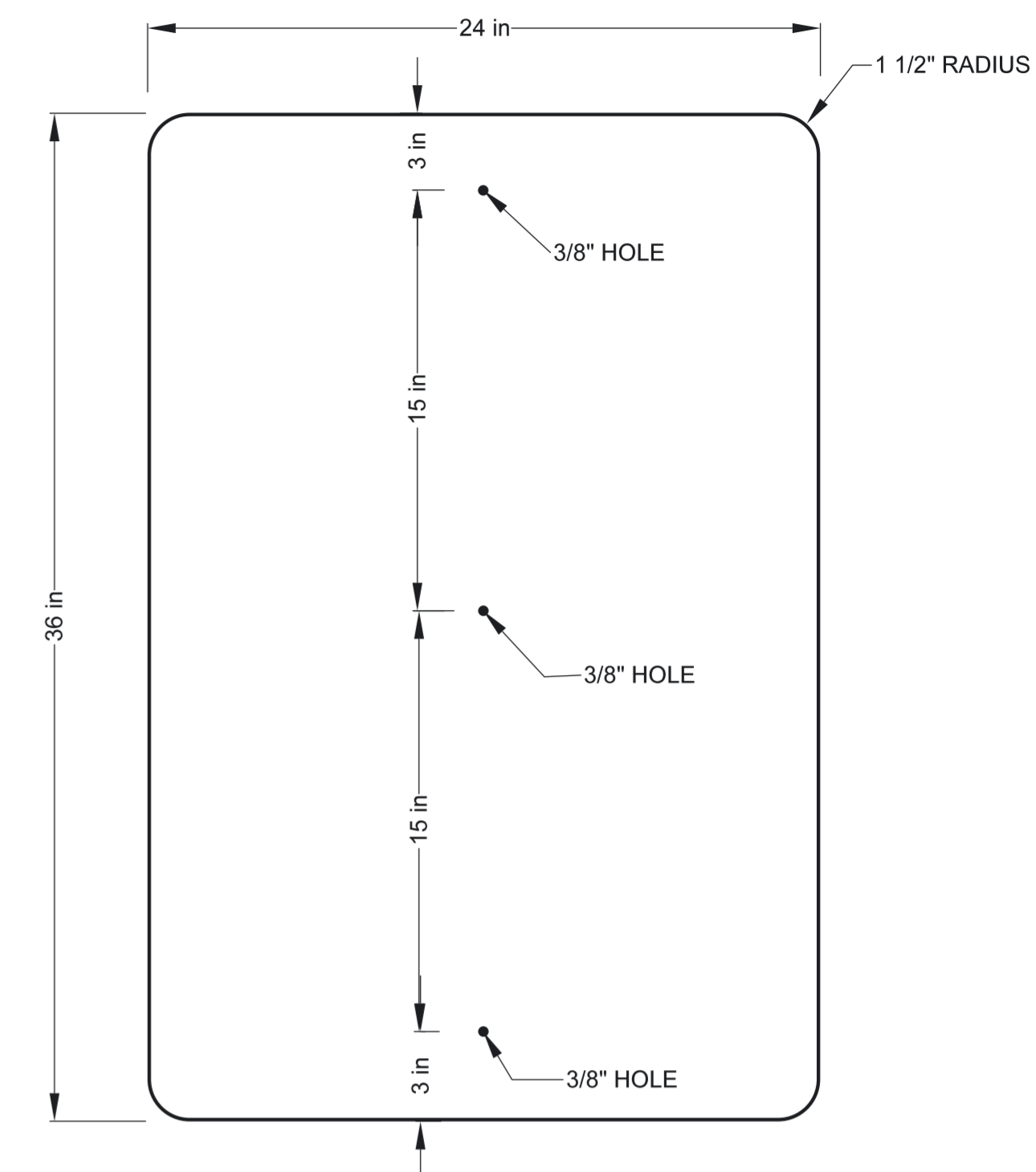
24" X 36" SIGN BLANK .080 GAUGE 3105 1 1/2" RADIUS-4 CORNERS 3/8" HOLES O.C.
