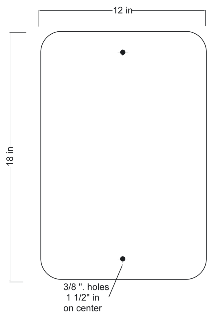
12" X 18" SIGN BLANK .080 GAUGE 3105 1 1/2" RADIUS-4 CORNERS 3/8" HOLES O.C.
