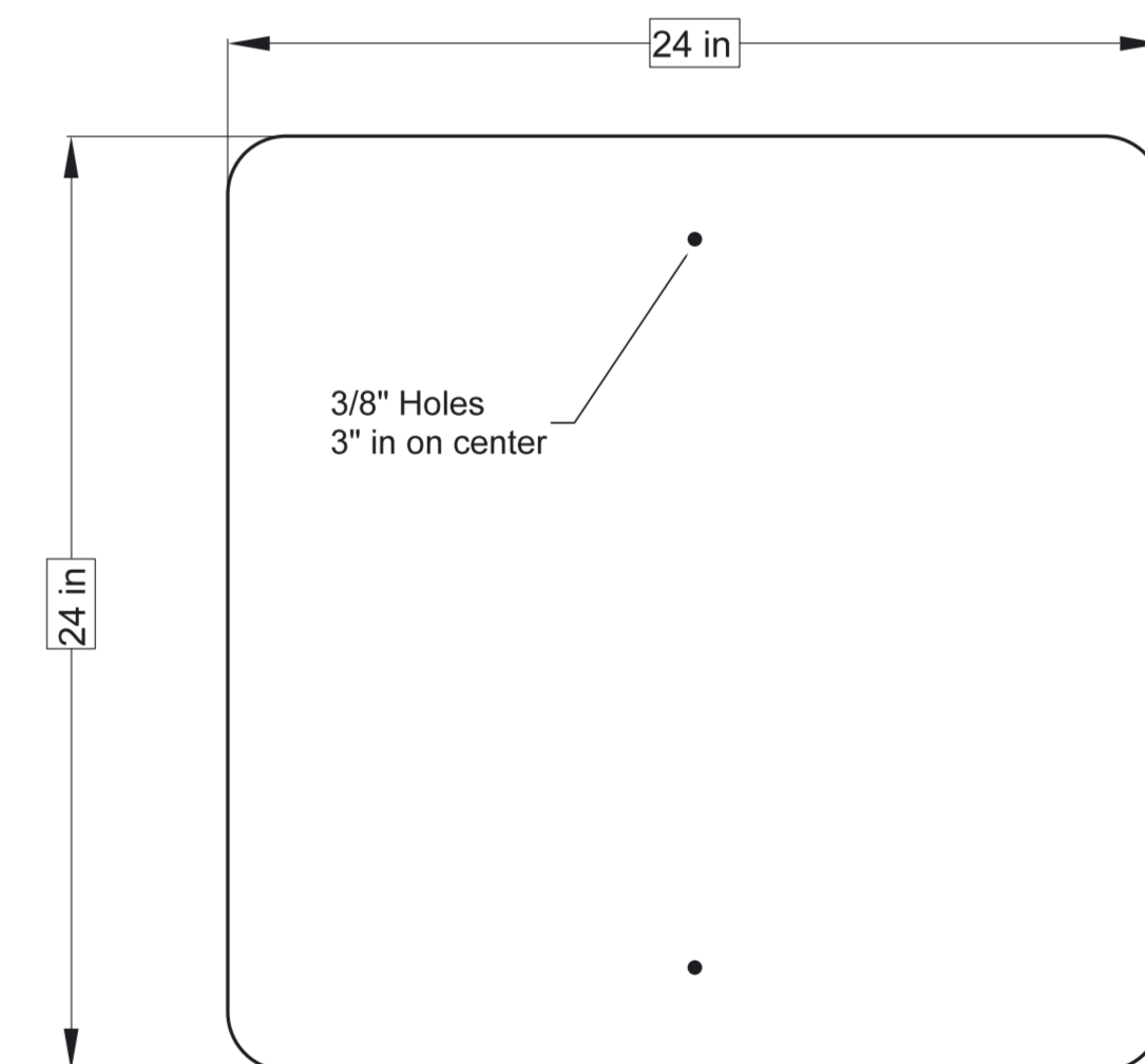
24" X 24" SIGN BLANK .080 GAUGE 3105 1 1/2" RADIUS-4 CORNERS 3/8" HOLES O.C.
