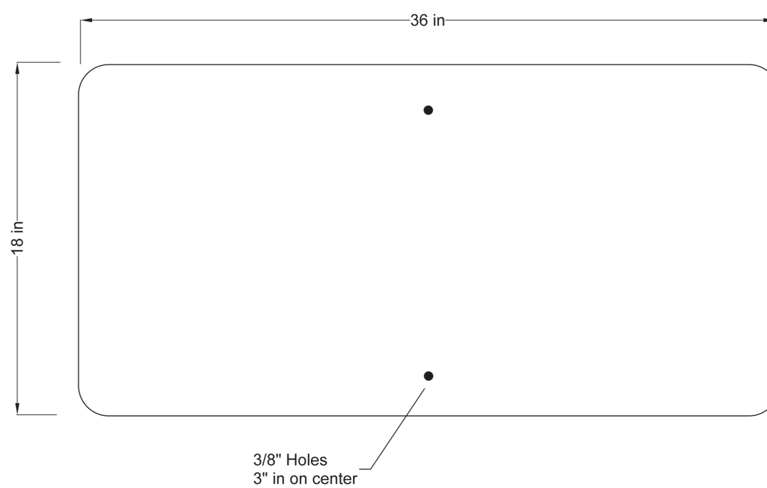
18" X 36" SIGN BLANK .080 GAUGE 3105 1 1/2" RADIUS-4 CORNERS 3/8" HOLES O.C.
