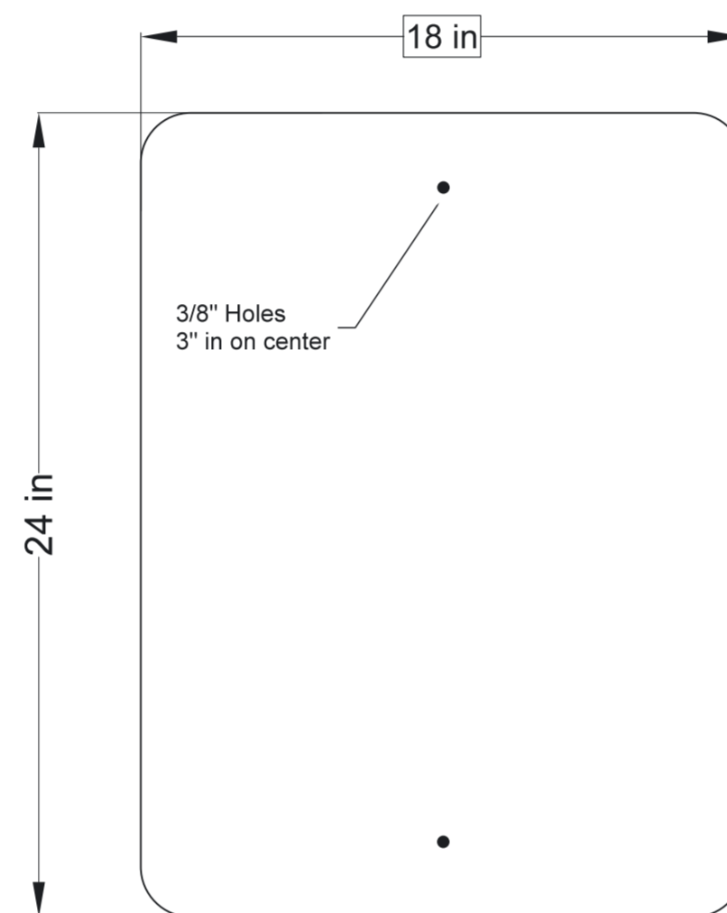
18" X 24" SIGN BLANK .080 GAUGE 3105 1 1/2" RADIUS-4 CORNERS 3/8" HOLES O.C.
