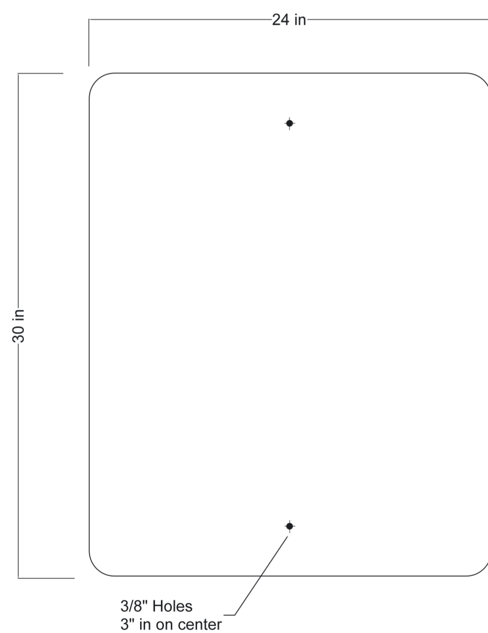
24" X 30" SIGN BLANK .080 GAUGE 3105 1 1/2" RADIUS-4 CORNERS 3/8" HOLES O.C.
