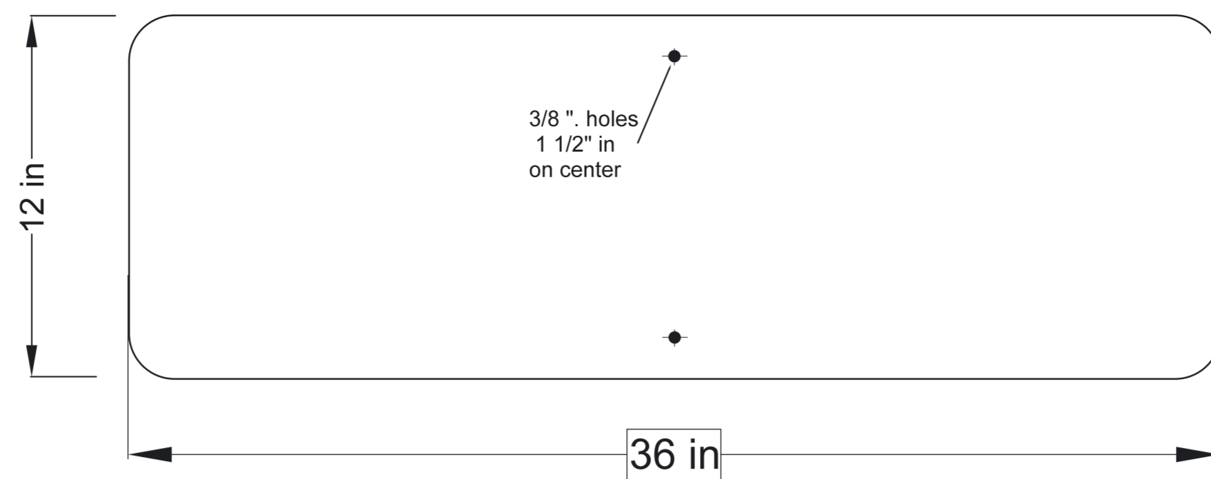
12" X 36" SIGN BLANK .080 GAUGE 3105 1 1/2" RADIUS-4 CORNERS 3/8" HOLES O.C.
