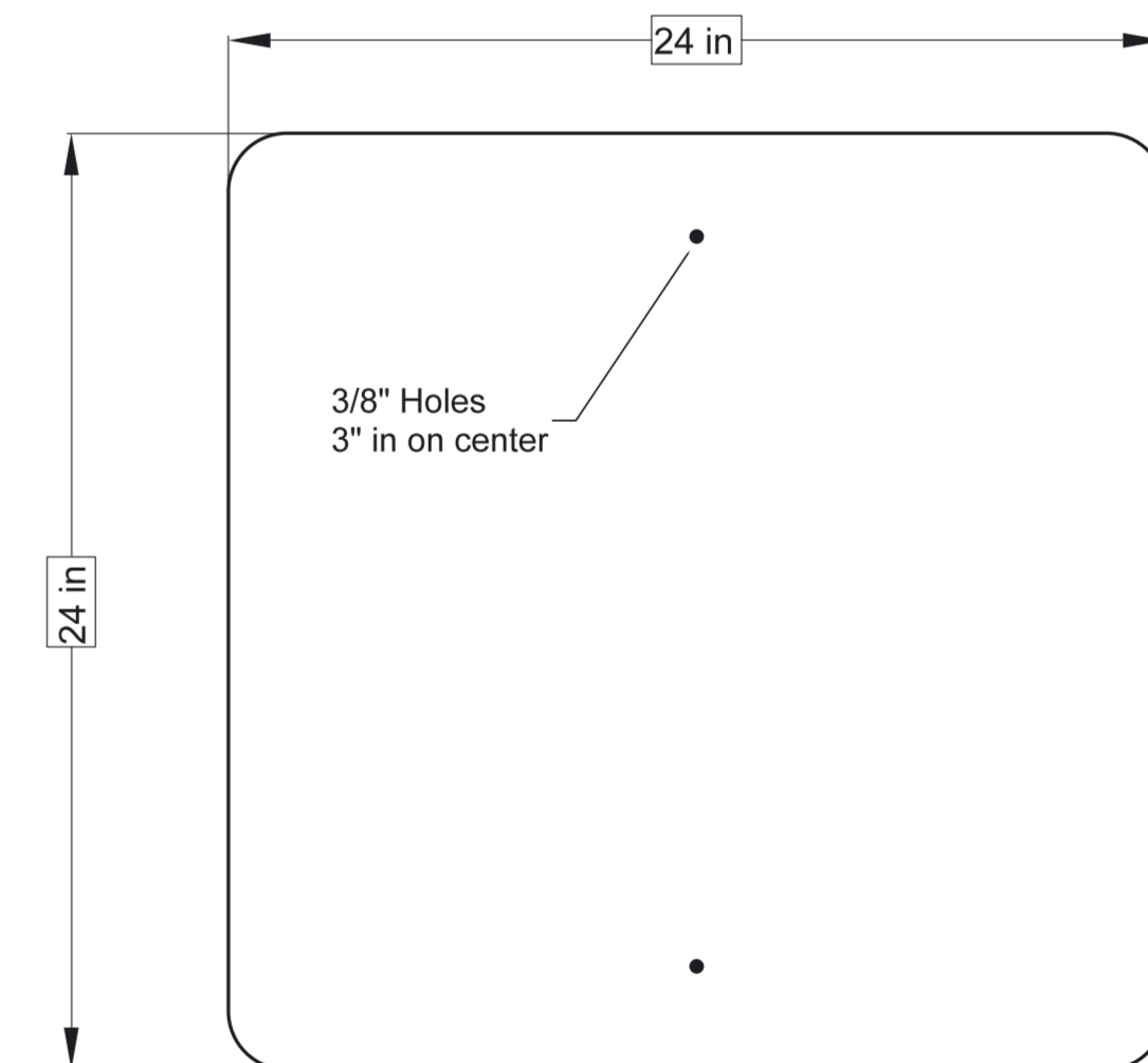
24" X 24" SIGN BLANK .080 GAUGE 3105 1 1/2" RADIUS-4 CORNERS 3/8" HOLES O.C.
