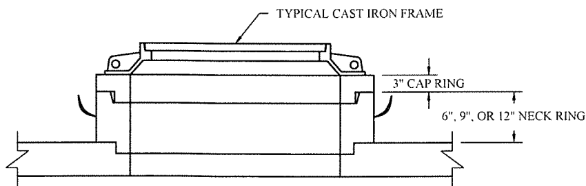
CAP/NECK RING ELEVATION DETAIL
