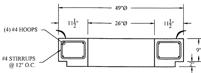
OPTIONAL REDUCING CAP RING
